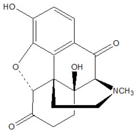
10-Ketooxymorphone
