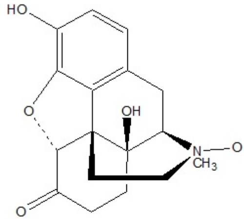
Oxymorphone N-oxide
