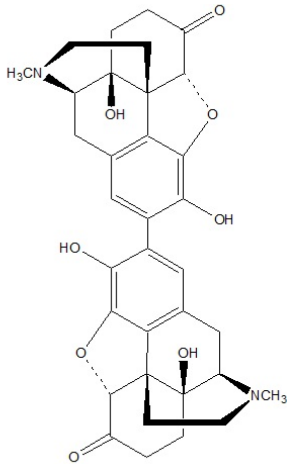
2,2'-Bisoxymorphone
